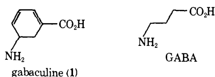
Figure 1. The reaction of gabaculine with equimolar amounts of pyridoxal phosphate. Aliquots (0.1 mL) of a 0.2 M potassium phosphate buffer (pH 7.0 at 25 °C) containing 10 mM gabaculine and 10 mM pyridoxal phosphate were placed in 1-mL screw cap Pyrex test tubes. The individual tubes were saturated with nitrogen, capped, and wrapped in aluminum foil. The tubes were placed in a boiling water bath and at the indicated times the test tubes were removed and the concentrations of gabaculine, pyridoxal phosphate, and CPP P were determined. B 6 refers to pyridoxal phosphate.
