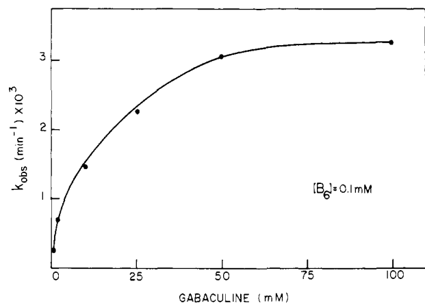
Figure 5. The pseudo-first-order rates of reaction of gabaculine with pyridoxal phosphate. These experiments were run similarly to those run in Figure 1 except that the starting concentration of pyridoxal phosphate was 0.1 mM and the concentrations of gabaculine used were 1, 3, 10, 25, 50, and 100 mM. In addition the temperature was maintained at 70 °C. The kinetics of the reactions were followed by measuring the amount of pyridoxal phosphate remaining by the phenylhydrazine method. 7 Rates of the reactions were determined at each concentration and the t_{1/2} values determined. The pseudo-first-order rate constants were determined from k_{\text{obsd}} = 0.693/t_{1/2} . In this figure pyridoxal phosphate is referred to as B_6 .
