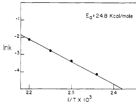
Figure 7. Arrhenius plot for the pseudo-first-order reaction of pyridoxal phosphate and gabaculine. From the previous experiment the k_{\text{obsd}} values were calculated. These values were plotted in the usual way to give the plot shown in this figure. The slope of the line gives -E_a/R and E_a calculates out to equal 24.8 kcal/mol.
