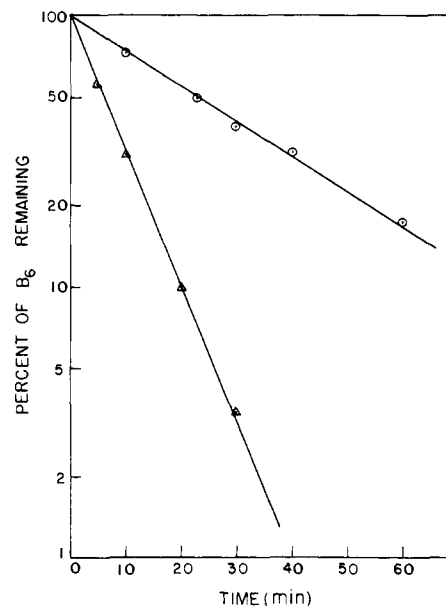
Figure 8. Deuterium isotope effect on the rate of adduct formation. Gabaculine and 4,5-dideuteriogabaculine (both at 10 mM) were heated together (80%) with pyridoxal phosphate at 0.1 mM. At the indicated times the pseudo-first-order rates of pyridoxal phosphate consumption were determined in the presence of gabaculine ( \Delta ) and dideuteriogabaculine ( \circ ). Knowing that 90% of the 5 position of dideuteriogabaculine contains deuterium the k_H/k_D calculates out to be 4.26.
