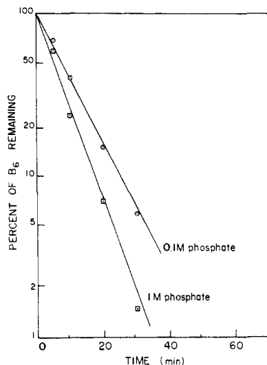
Figure 9. Buffer catalysis on the rate of the reaction. At 70 °C the rates of the reaction between pyridoxal phosphate at 0.1 mM and gabaculine at 100 mM were measured in 0.1 and 1 M potassium phosphate buffer at pH 7.0. The ionic strength was maintained the same in both cases by the addition of potassium chloride. The rates of the reactions were determined by following the rate of disappearance of pyridoxal phosphate with phenylhydrazine. 7
