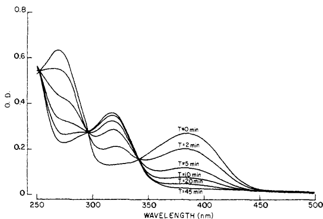
Figure 2. Ultraviolet spectral changes accompanying the reaction of gabaculine and pyridoxal phosphate. This experiment was run identically with the one above; at the indicated times the ultraviolet spectrum of the content of each test tube was determined. Gabaculine itself has \lambda_{\max} at 275 nm and \log \epsilon = 3.93 .
