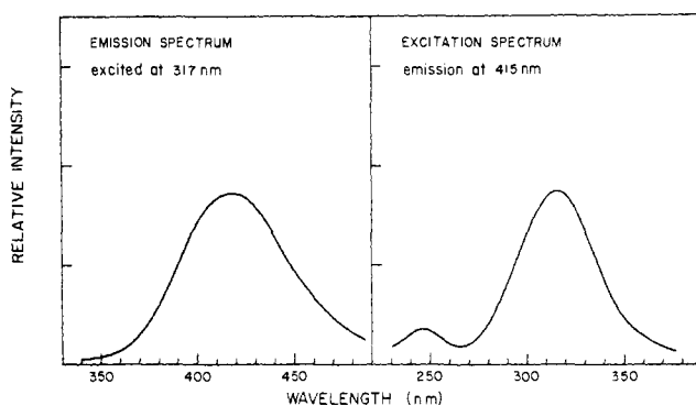
Figure 4. The fluorescence excitation and emission spectra of \text{CPP}_p . A 5 \times 10^{-6} M solution of \text{CPP}_p on the above buffer was made up. The excitation and emission spectra were determined 1-cm pathlength cells. The spectra are given as recorded and are uncorrected.
