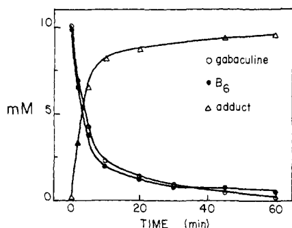
Figure 1. The reaction of gabaculine with equimolar amounts of pyridoxal phosphate. Aliquots (0.1 mL) of a 0.2 M potassium phosphate buffer (pH 7.0 at 25 °C) containing 10 mM gabaculine and 10 mM pyridoxal phosphate were placed in 1-mL screw cap Pyrex test tubes. The individual tubes were saturated with nitrogen, capped, and wrapped in aluminum foil. The tubes were placed in a boiling water bath and at the indicated times the test tubes were removed and the concentrations of gabaculine, pyridoxal phosphate, and CPP P were determined. B 6 refers to pyridoxal phosphate.
