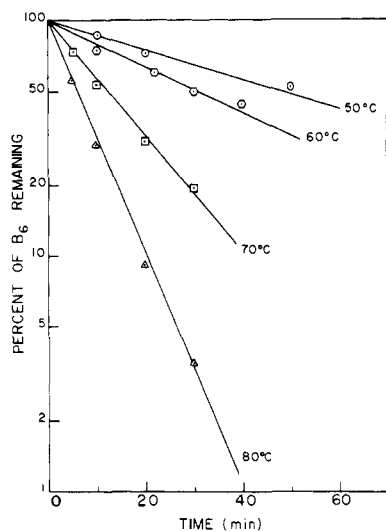
Figure 6. The effect of temperature on the pseudo-first-order rate of the reaction of gabaculine with pyridoxal phosphate. These experiments were conducted with pyridoxal phosphate at 0.1 mM and gabaculine at 100 mM. For each temperature the rates of disappearance of pyridoxal phosphate were measured. The reactions were conducted at 50, 60, 70, and 80 °C.
