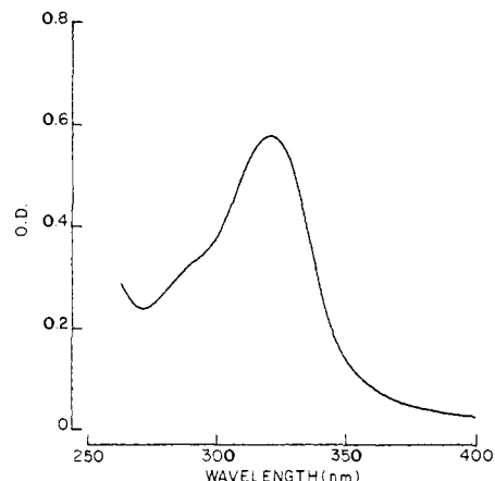
Figure 3. The ultraviolet spectrum of \text{CPP}_p . The ultraviolet spectrum of a 1.07 \times 10^{-4} M solution of \text{CPP}_p in 0.2 M potassium phosphate (pH 7.0) was recorded. The \lambda_{\max} is at 320 nm with \log \epsilon = 3.74 .
